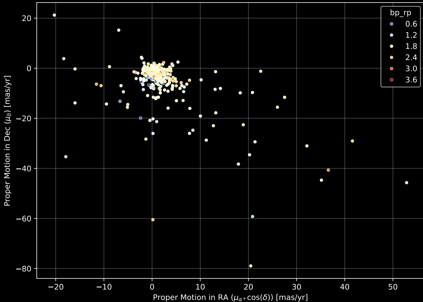
APOGEE DR17 Field: [180-04] Proper Motion Diagram (n= 418)
