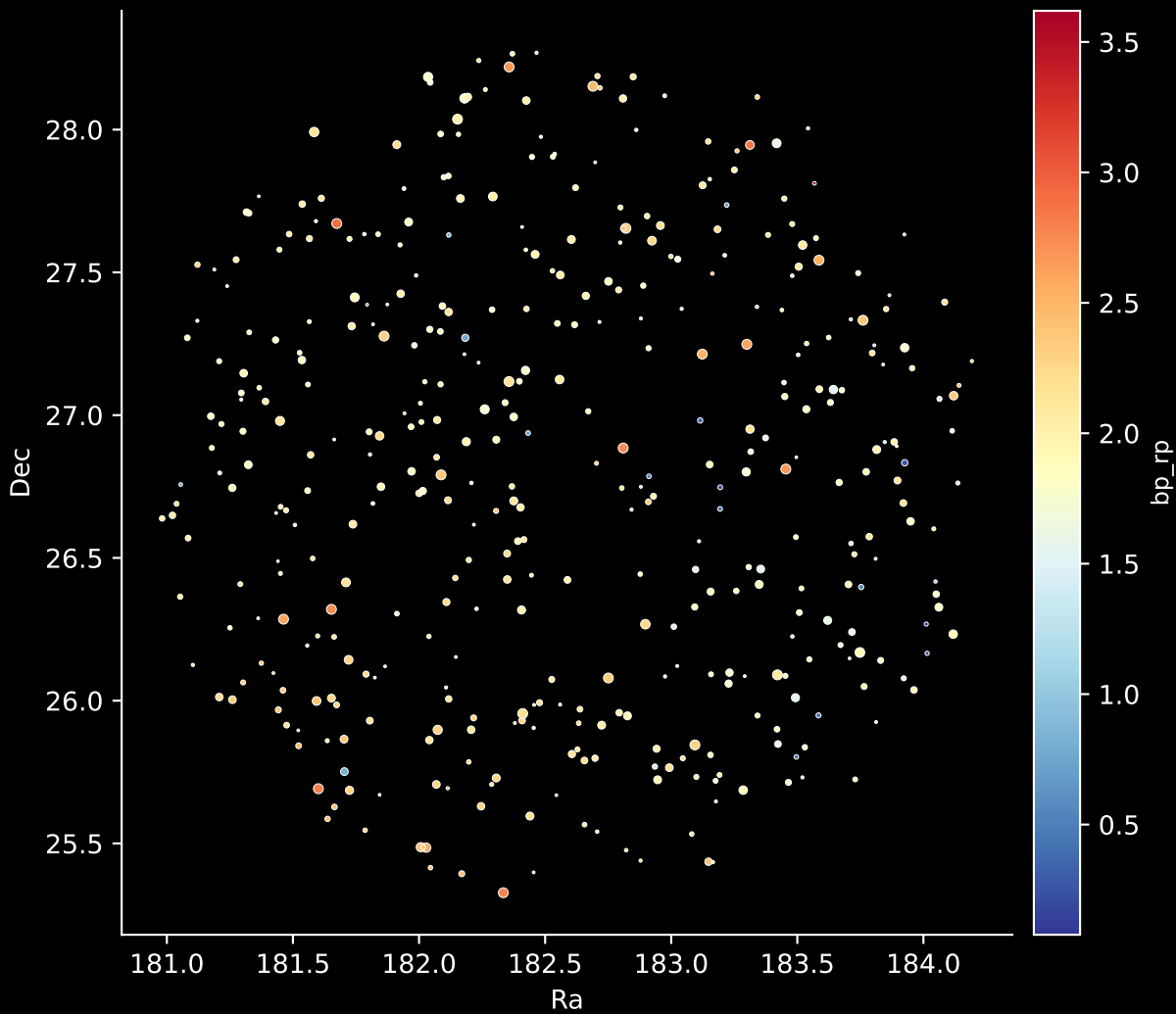
APOGEE DR17 Field: [180-04] Stars: 418
