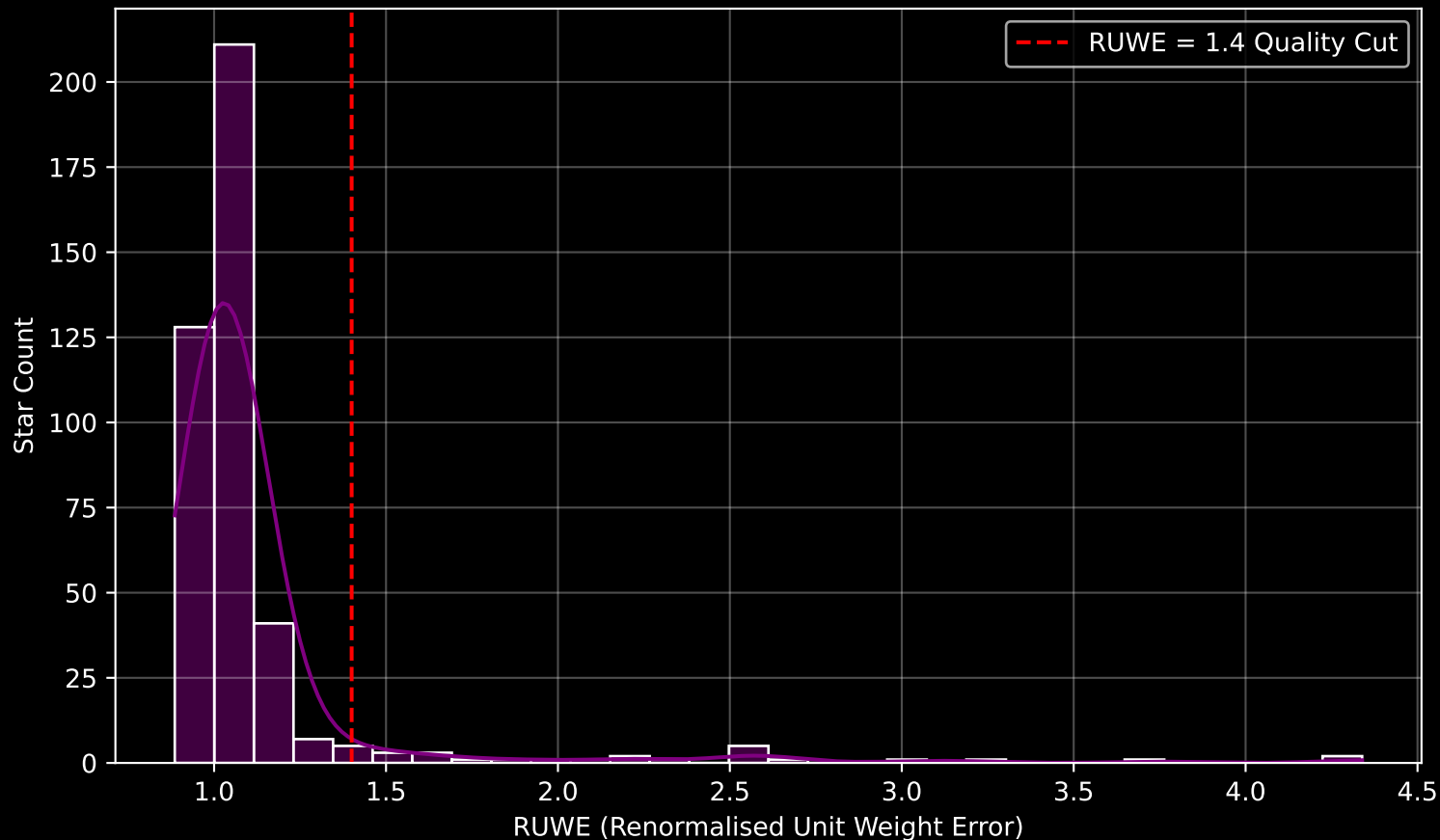
GAPOGEE DR17 Field [180-04] RUWE Distribution (n= 415)
