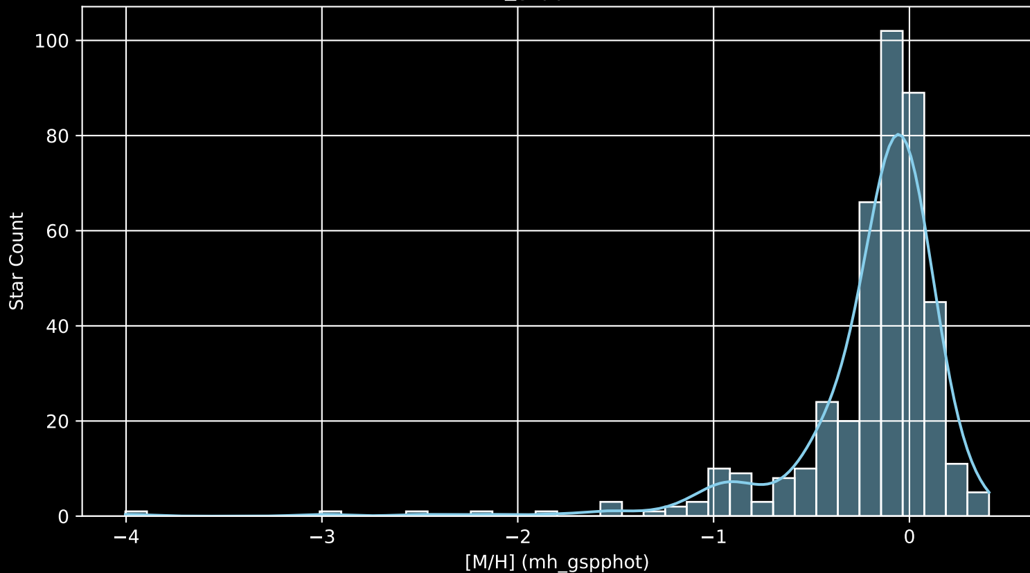
APOGEE DR17 Field: [180-04 [M/H] (mh_gspphot) (n= 416)
