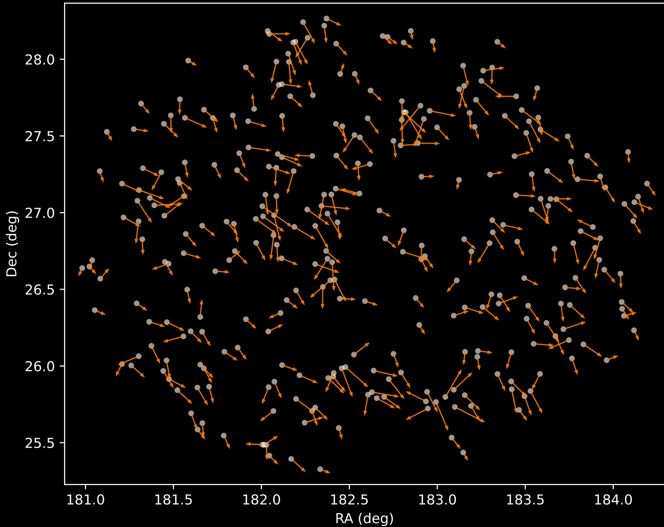
APOGEE DR17 Cluster 2 Proper Motion Vectors (n=304)
