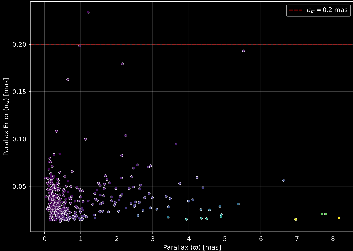
APOGEE DR17 Field: [180-04] Parallax Quality (n= 418)
