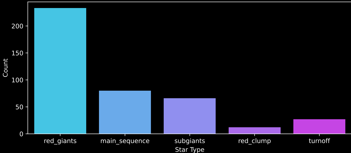
APOGEE DR17 Field: [180-04] Count plot of Star Type
